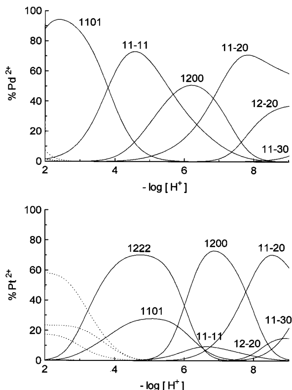
Fig. 5 Distribution diagrams of complexes formed in the \text{Pd}^{\text{II}} -Gly-Gly-( P ) (upper) and \text{Pt}^{\text{II}} -Gly-Gly-( P ) (lower) systems as a function of -\log[\text{H}^+] ( c_{\text{M}} = 0.005 , c_{\text{H}_2\text{A}} = 0.01 \text{ mol dm}^{-3} ). The dashed curves belong to chloro-complexes. Numbering of the species corresponds to the molar ratio \text{M}:\text{A}:\text{H}:\text{Cl}
