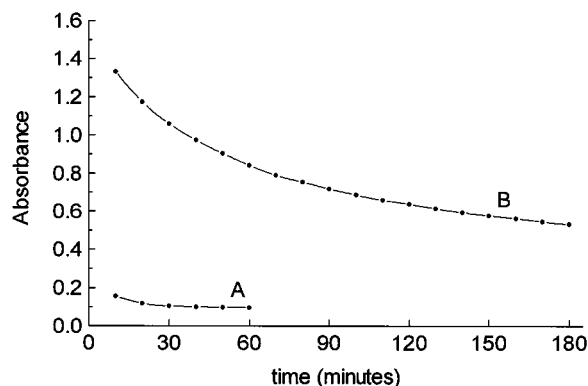
Fig. 1 Dependence of absorbance on time in the system Pd II -Gly-Gly-( P ), c_{\text{Pd}} = 0.0015 \text{ mol dm}^{-3} ( \text{M}:\text{H}_2\text{A} = 1:2 ), \lambda = 305 \text{ nm} , pH after 3 d: A, pH 4.2; B, pH 9.1
