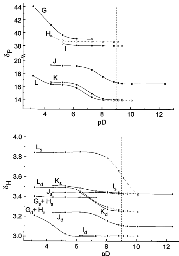
Fig. 8 Variation of \delta_P vs. pD (upper) and \delta_H (lower) for the \text{Pd}^{\text{II}} -Gly-Gly-(P) system. Key as in Fig. 7. Curves G corresponds to deprotonation of the phosphonic group in species 1101 and formation of 11-11, H (low abundance) to 11-10, I to 11-20, J to deprotonation of phosphonic groups in 1200 and formation of 12-20, K to species co-ordinated only through the amine group, i.e. 1222 2N , 1200 2N and 12-20 2N and A to free Gly-Gly-(P). Subscripts s and d correspond to the methylene in Gly and Gly-(P) parts of the molecule
