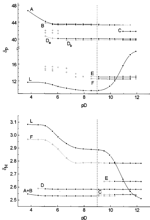
Fig. 7 Variation of \delta_P vs. pD (upper) and \delta_H (lower) for the \text{Pt}^{\text{II}} -Gly-(P) system. Open circles indicate species of low relative abundance, the broken vertical line the region of pH used for data treatment. Curve A corresponds to deprotonation of phosphonic group in species 1112 and formation of 1102, B to 1100, C to 11-20, D to 1200 ( D_a , D_b = probable cis , trans isomers), E to 11-30, F to species co-ordinated only through the amine group, i.e. 1222 2N , 1202 2N , 1200 2N and 12-20 2N , and A to free Gly-(P)
