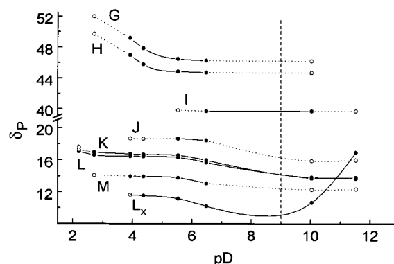
Fig. 9 Variation of \delta_P vs. pD for the \text{Pt}^{\text{II}} -Gly-Gly-(P) system. Empty circles indicate species of low relative abundance. Curves G belong to deprotonation of the phosphonic group in species 1101 and formation of 11-11, H to 11-10, I to 11-20, J to deprotonation of phosphonic groups in 1200 and formation of 12-20, K to species co-ordinated only through the amine group, i.e. 1222 2N , 1200 2N and 12-20 2N , A to free Gly-Gly-(P), L_x to Gly-(P) after hydrolysis of the peptide bond and M to a complex of \text{Pt}^{\text{II}} with Gly-(P)
