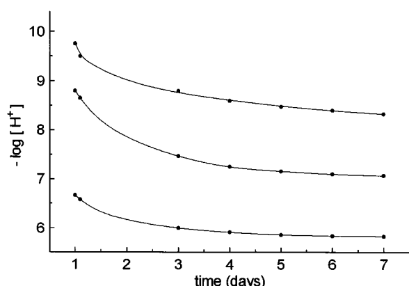
Fig. 2 Dependence of pH on time in the system Pt II -Gly-( P ), c_{\text{Pt}} = 0.005 \text{ mol dm}^{-3} ( \text{M}:\text{H}_2\text{A} = 1:2 )
